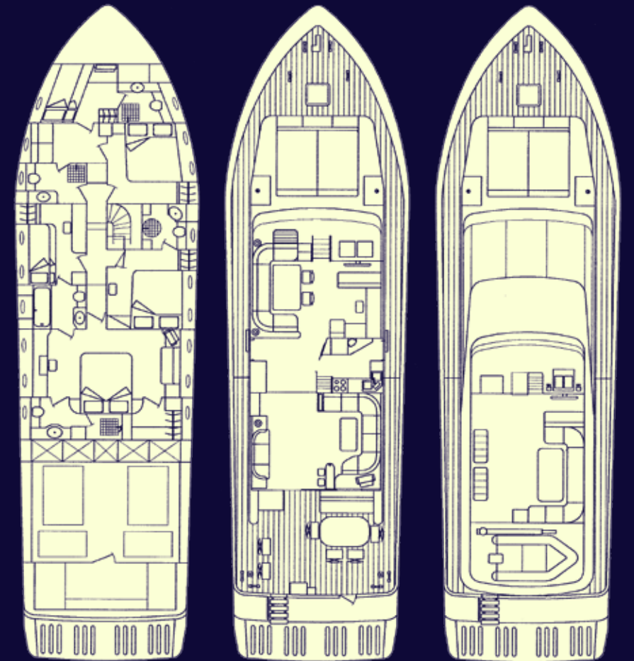
Lower Deck
